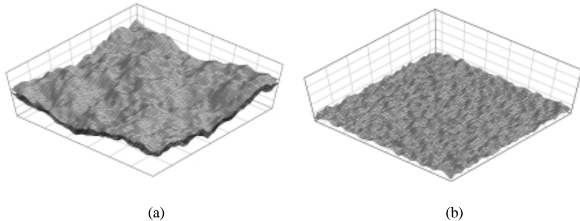
Fig. 3 Typical synthetic fracture models produced with SynFrac™ software. (a) Upper and lower bounding surfaces of the fracture. (b) Resulting aperture variation across the fracture. Note that the lack of long wavelength in the aperture. This is the result of the fracture surfaces being matched at the larger wavelength.
