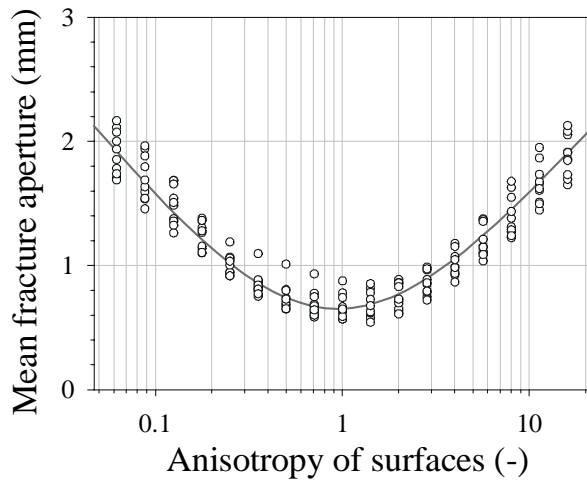
Fig. 6 Mean synthetic fracture aperture as a function of the anisotropy of surfaces. Fractal dimension 2.1, mismatch length 10 mm, transition length 20 mm, standard deviation of surfaces 0.5 mm.
