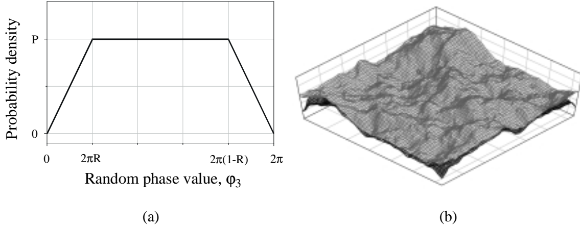
Fig. 2 Numerical model of rough fractures by Glover et al. (1998). (a) Non-uniform probability density distribution of random phase \varphi_3 . (b) Sample of synthesized numerical fracture. Non-uniform distribution of phases causes aperture increasing at the corners.
