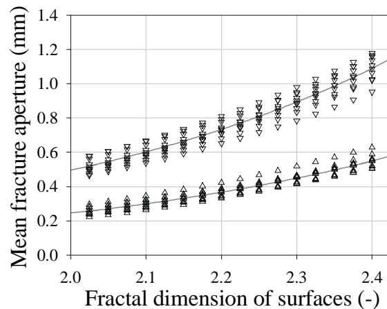
Fig. 5 Mean synthetic fracture aperture as a function of the fractal dimension of surfaces. Mismatch length 10 mm, transition length 20 mm, standard deviation of surfaces 0.3 mm ( \Delta ) and 0.6 mm ( \nabla ).
